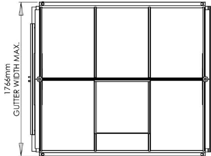
5 X 6 REGATTA DWARF
